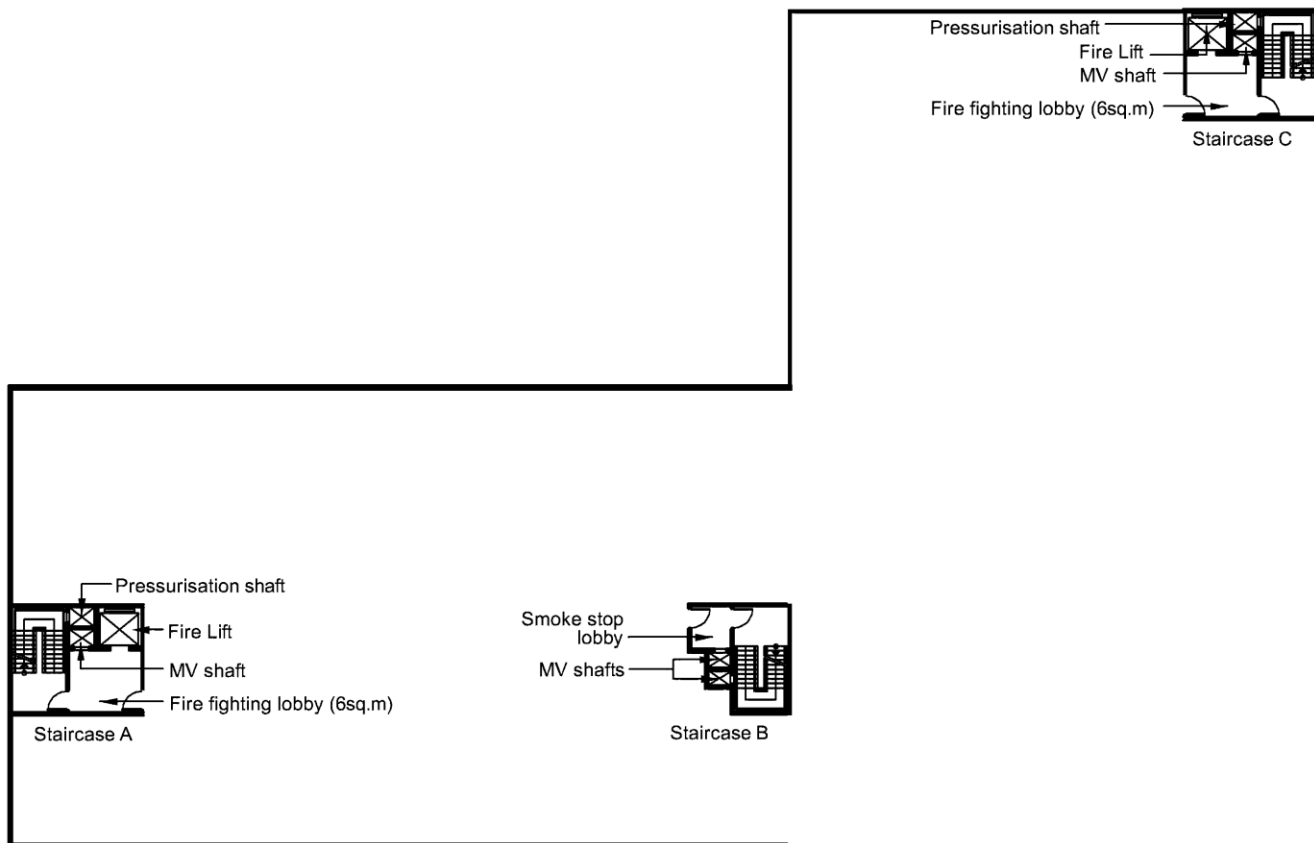
Typical Basement Plan (> 4 basement storey)
