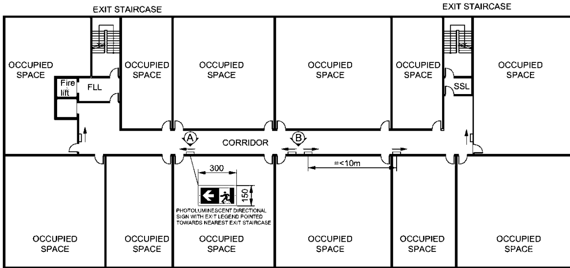
PLAN VIEW: PL SIGNS FOR INTERNAL CORRIDOR
