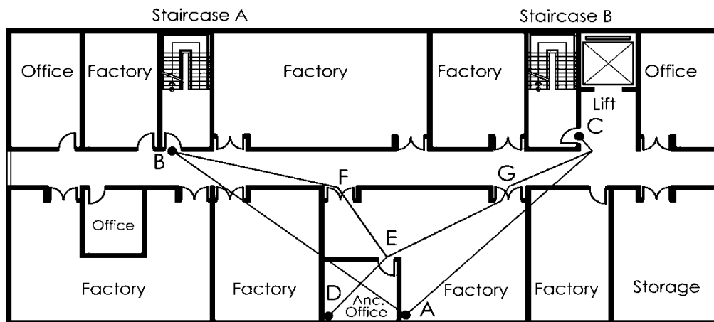
Example of a mixed development with factory, office and storage
