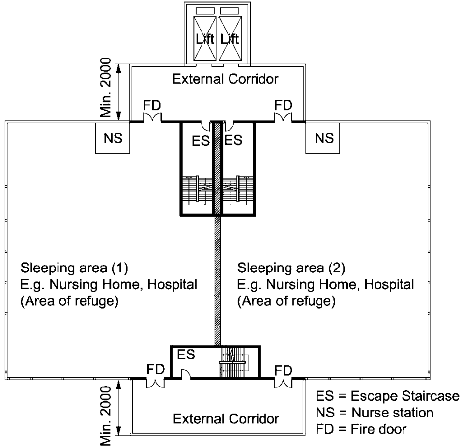
Example (2) of health care occupancy layout
