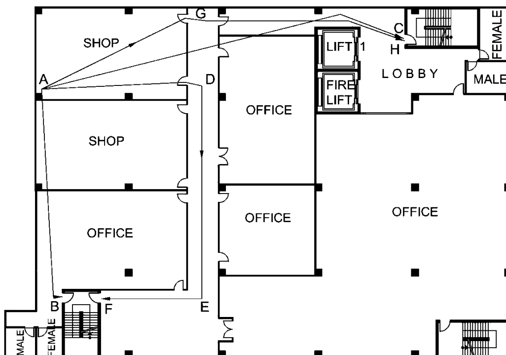
AB and AC are Direct Distance measurement paths annotated by \longleftrightarrow ADEF and AGH are Travel Distance measurement paths annotated by \dashleftarrow Diagram 2.2.2-6
