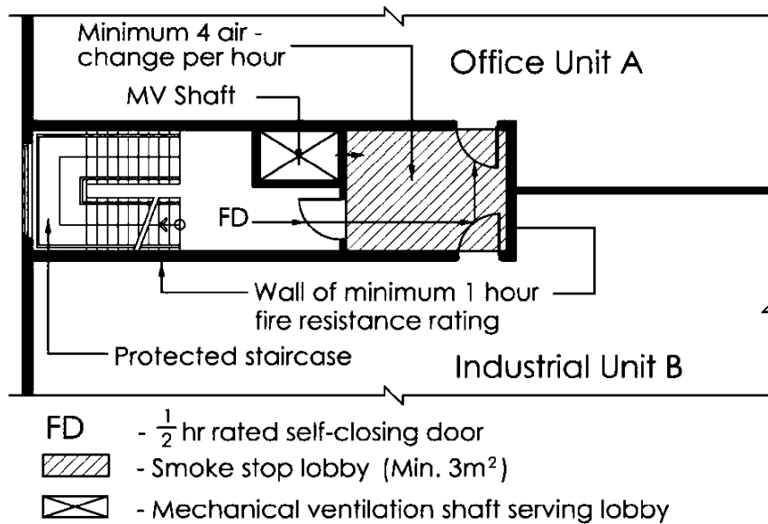
Mechanically Ventilated Smoke Stop Lobby
