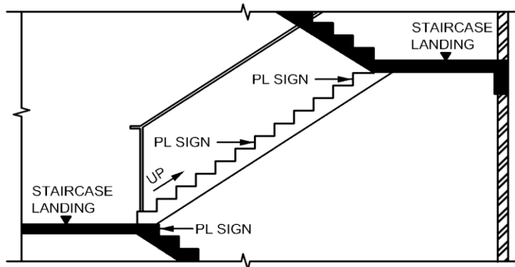
TYPICAL SECTION STAIRCASE FLIGHT IN BASEMENT
