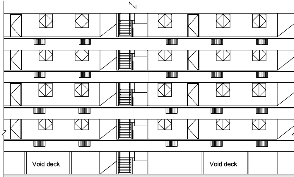
Elevation view
