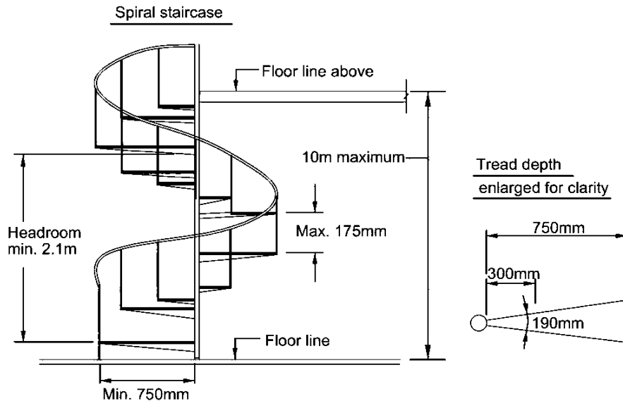
Tread depth enlarged for clarity
