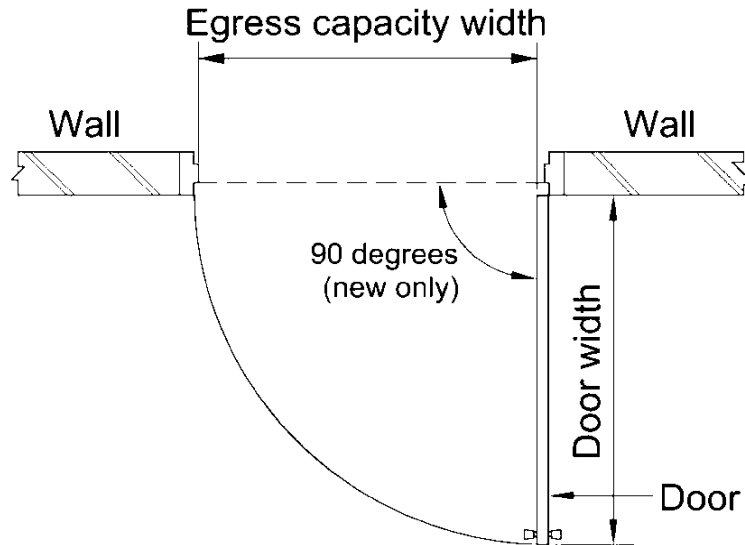
Minimum clear width
