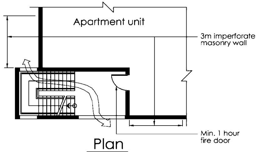
Diagram 2.2.13(c) (i)(3) & 2.2.13(c)(ii)
