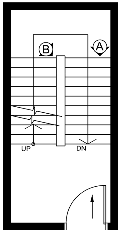
TYPICAL FLOOR PLAN VIEW
