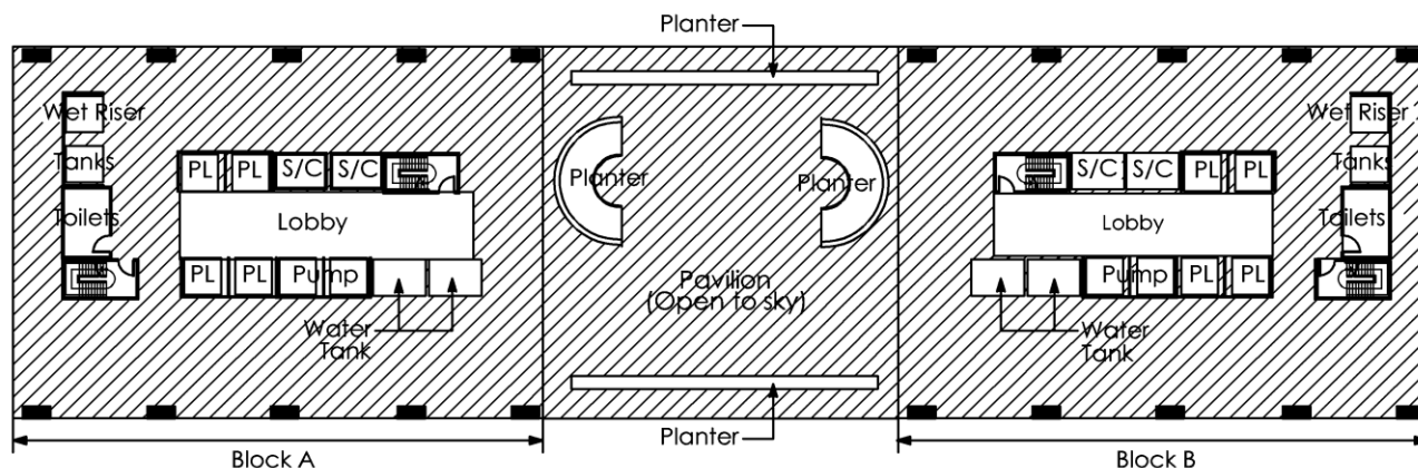
Examples of Non-simultaneous areas
