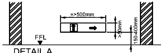
DETAIL A PL TAPE WITH DIRECTIONAL ARROW & EXIT LEGEND ON STAIRCASE LANDING WALL
