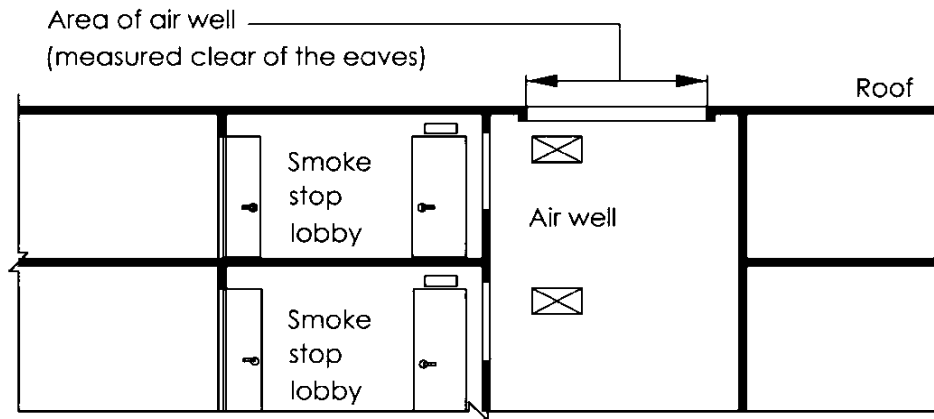
Sectional view
