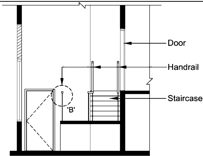
Sectional Elevation
