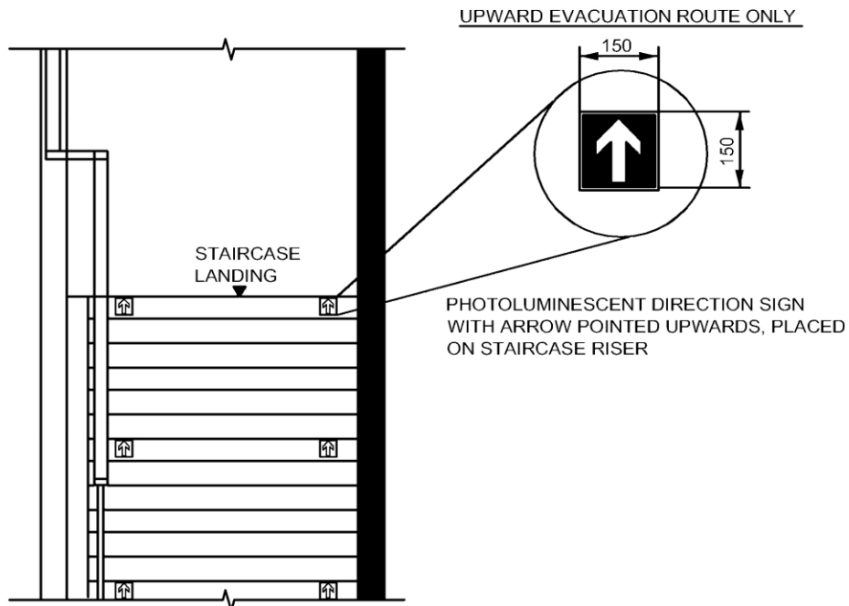
DETAIL A FRONT ELEVATION
